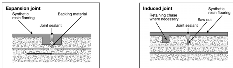
Figure 1: Movement joints
